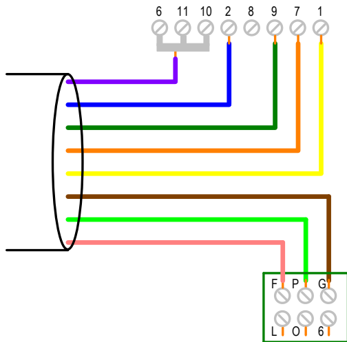
Old style 1130/NID handset connections
