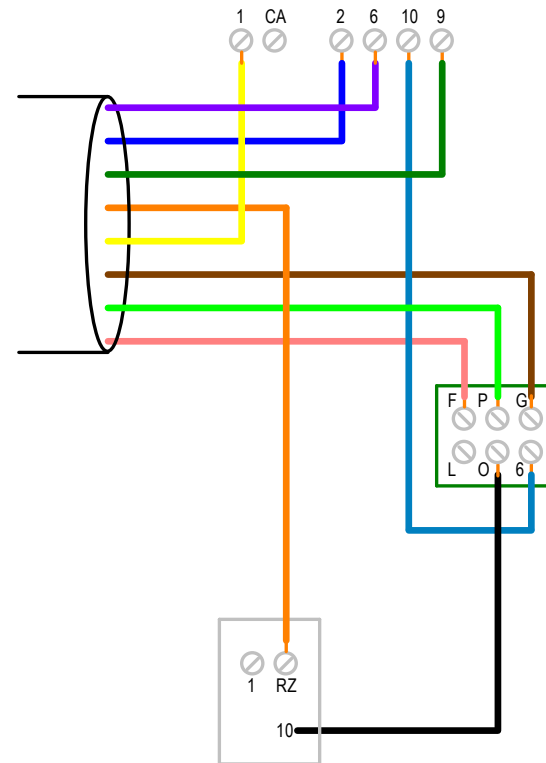
New style 1130/NID handset connections
